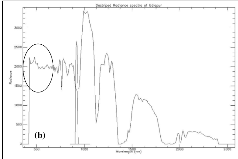
Figure 5-2 Local balancing effect of de-stripping on the image spectra taken over know bad column. The encircled region shows the region of improvement. (a) spectra of Level 1 R product (b) spectra after de-stripping.
