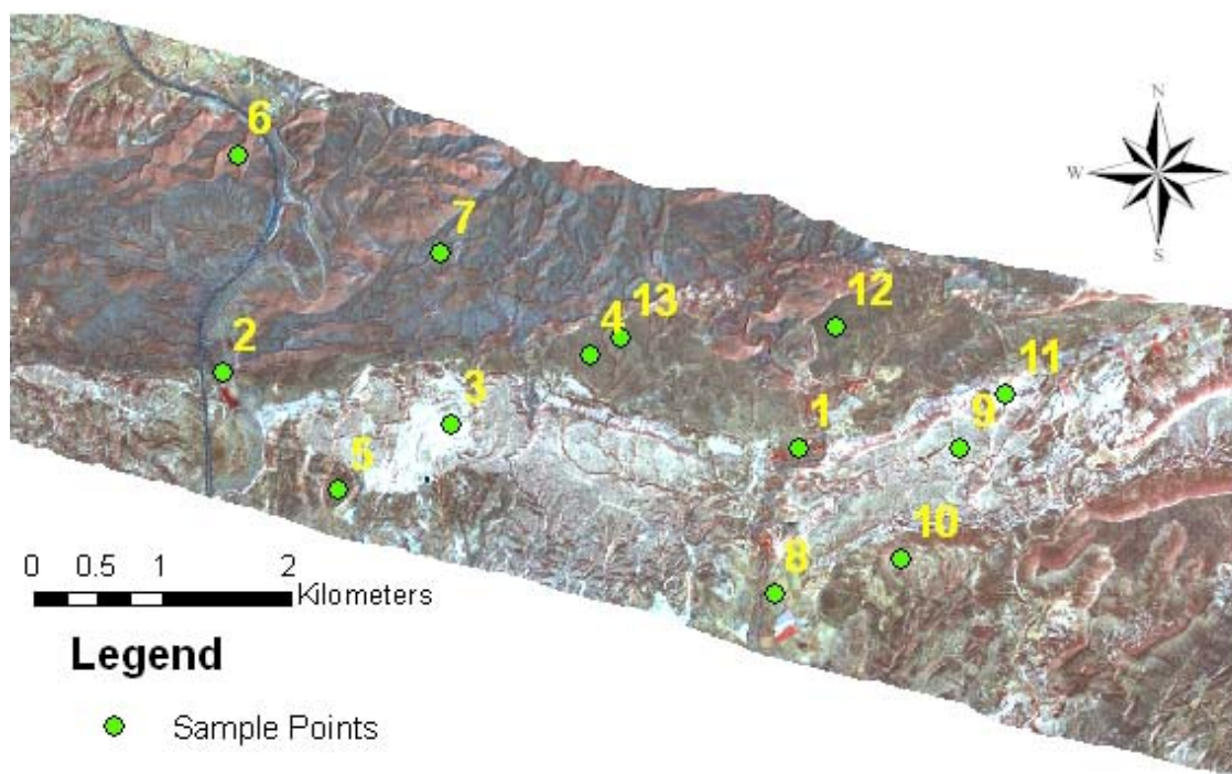
Figure 4-5 HyMap image of Rodalquilar, Spain showing location of sample points collected for creation of spectral library
