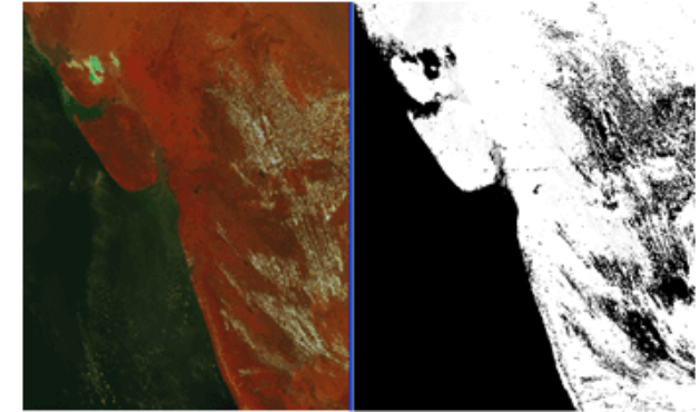
Cloud masking using OCM bands
